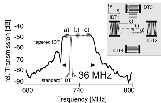
FIG. 1. Frequency response of a tapered IDT. The variation of the finger period over the transducer aperture spreads the IDT frequency response to a bandpass of 36 MHz width. For comparison, the transmission of an untapered IDT is also shown. A schematic sample layout is sketched in the inset.
