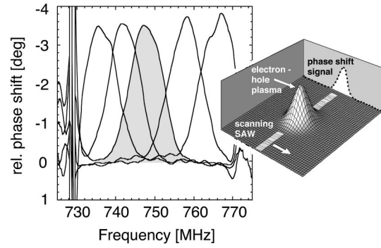
FIG. 2. Images of a photogenerated electron hole plasma at different laser spot positions within the tapered IDTs "field of view." The hatched trace corresponds to the fitting parameters given in the text. The inset schematically explains the origin of the phase signal.
