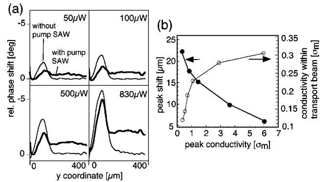
FIG. 4. (a) Phase shift image of the laser spot and the acoustic transport tail for various laser intensities. (b) Drag of the laser spot core (closed circles) and conductivity in the charge transport tail (open circles) vs conductivity in the core region. Dynamic screening at high carrier densities reduces both the drag of the EHP core and the transport efficiency. The latter is expressed by a saturation of the conductivity in the transport tail.
