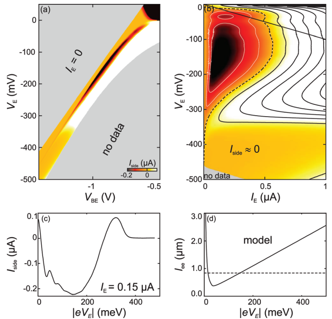
FIG. 4. (Color online) (a) I_{\text{side}} as a function of V_{BE} and V_E measured for dissipated powers |V_E \times I_E| \leq 700 nW. No data exist for higher powers (lower right corner) and for the upper left corner; here the emitter QPC is closed and all currents vanish. (b) Same data as in (a), plotted as a function of injected current, I_E ; contour lines are spaced by 70 nA, I_{\text{side}} \approx 0 is marked by a dashed line. (c) Vertical slice of Fig. 4(a) at I_E = 0.15 \mu\text{A} ; (d) numerical calculations of electron-electron scattering length, l_{ee} , as a function of excess kinetic energy |eV_E| \simeq E_{\text{kin}} - E_F at T=0 ; the dashed line marks sample dimensions.
