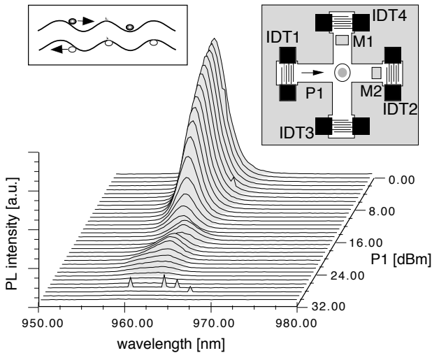
Fig. 1. Photoluminescence spectra on sample B at 5K for different acoustic powers. Electron-hole pairs are generated at the cross-center by a 780nm laser with an intensity of about 10mW/cm^2 . The insets schematically depict the sample design and the SAW field induced separation of the optically generated carriers.
